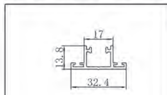
NAME CODE SLIP GROOVE FGT14003F
