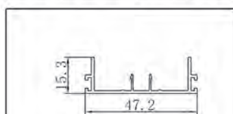
NAME CODE ASTRAGAL FGT14009
