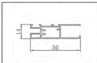
NAME CODE SCREEN PANEL F868S02
