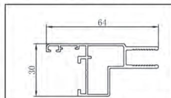
NAME CODE SCREEN PANEL F85S01
