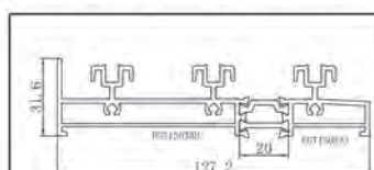
NAME CODE JAMB Moulding FGT13006
