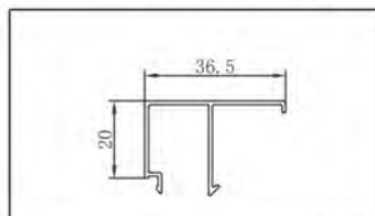
NAME CODE MOULDING F8505
