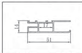
NAME CODE SCREEN PANEL F868S01
