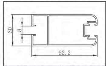
NAME CODE LOCKSTILE F86806
