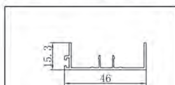
NAME CODE SCREEN Moulding FGT14005YX
