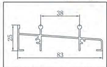
NAME CODE DOUBLE FLAT SILL F86812
