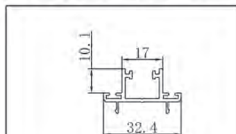
NAME CODE ASTRAGAL FGT14009
