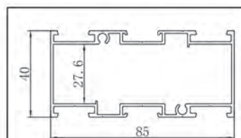
NAME CODE WINDOW PREMETER1.2 F8501
