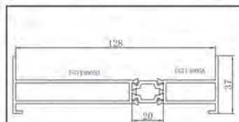
NAME CODE 3 TRACKS JAMB FGT13005
