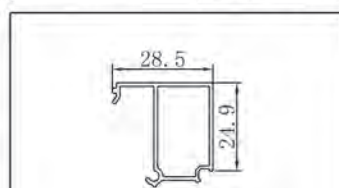
NAME CODE BIG Moulding S95432
