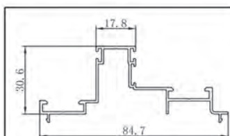
NAME CODE SUB FRAME F8503
