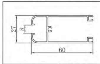
NAME CODE BOTTOM F86805A
