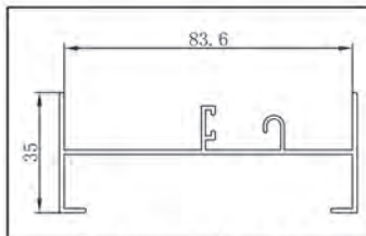
NAME CODE DOUBLE JAMB F86803
