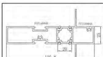
NAME CODE GLASS DIVIDER FGT13004
