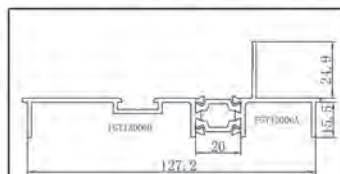
NAME CODE JAMB Moulding FGT13006
